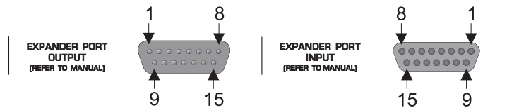
Fig. 4.8: Expander Port connectors
