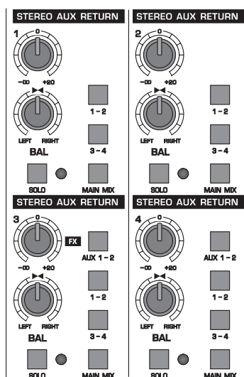
Fig. 2.12: Aux Return Main section
