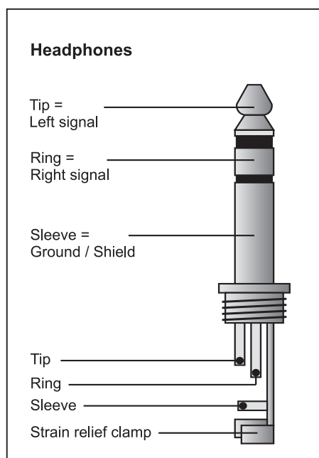
Fig. 6.1: Headphones connector
